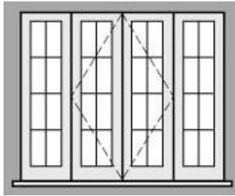
Eight Lite with fixed sidelites
